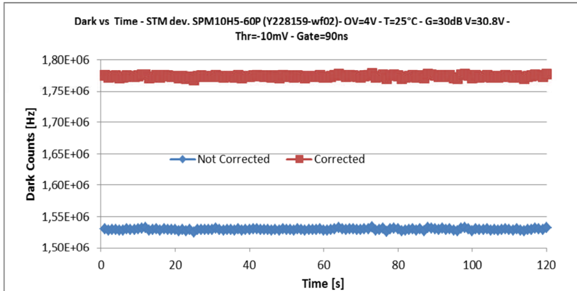
Fig.4 - DARK vs Time V_{ov}=4V - Thr=-10\text{ mV} T=25^\circ The upper curve is obtained correcting for dead time the lower curve. Temperature compensation for gain stabilization is also adopted.
