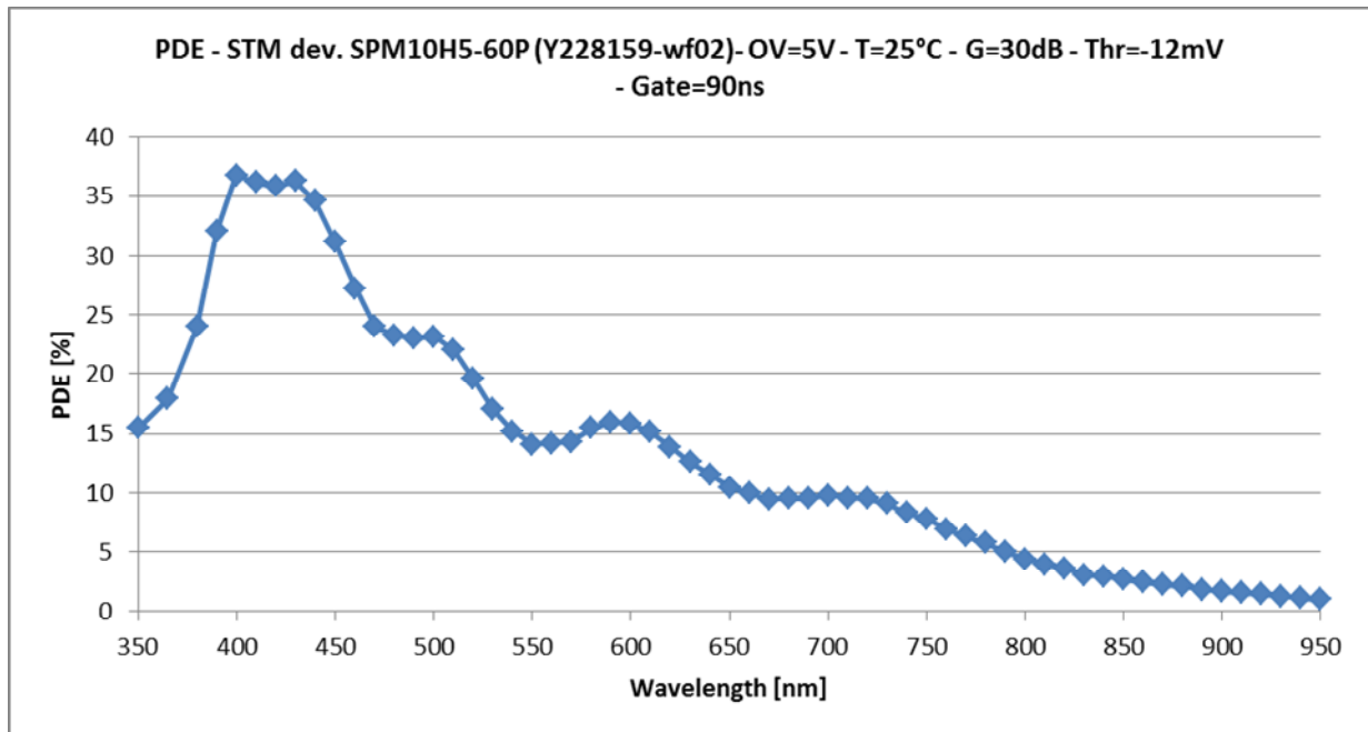
Fig.13 – PDE measurements operating the SiPM at V_{ov}=5V T=25^{\circ}C , V_{thr}=-12 mV, Gate time=90 ns
