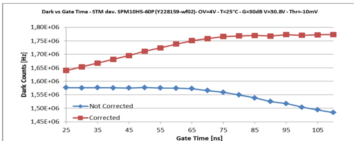
Fig.3 - DARK vs GATE TIME V_{ov}=4V - Thr=-10\text{ mV} T=25^{\circ} . Measurements were performed at gate times from 25ns to 110ns. The upper curve is obtained correcting for dead time the lower curve. Temperature compensation for gain stabilization is also adopted
