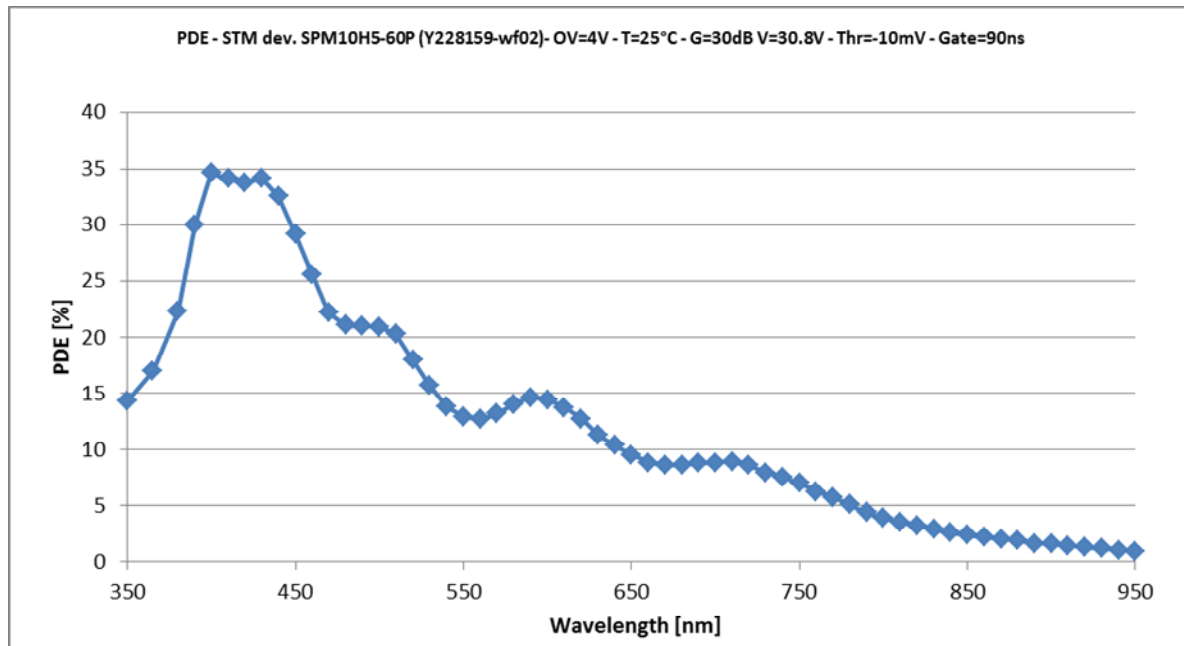
Fig.7 – PDE measurements operating the SiPM at V_{ov}=4V T=25^{\circ}C , V_{thr}=-10 mV, Gate time=90 ns
