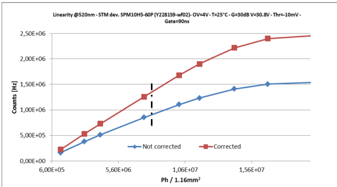
Fig. 5 – Linearity at 520 nm with and without the dead time correction.
