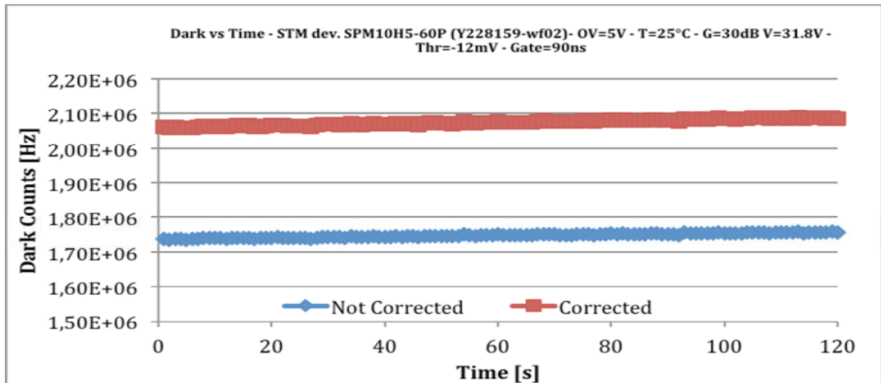
Fig.10 - DARK vs Time V_{ov}=5V - Thr=-12\text{ mV} T=25^\circ . The upper curve is obtained correcting for dead time the lower curve. Temperature compensation for gain stabilization is also adopted.
