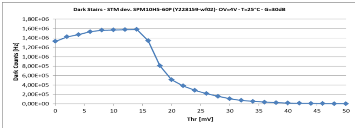
Fig. 2 – Dark Stair versus V_{thr} @ T=25.0^{\circ}C .
