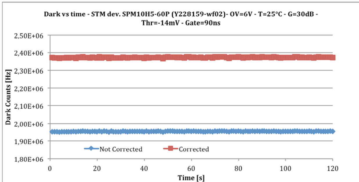
Fig.16 - DARK vs Time V_{ov}=6V - Thr=-14\text{ mV} T=25^\circ The upper curve is obtained correcting for dead time the lower curve. Temperature compensation for gain stabilization is also adopted.
