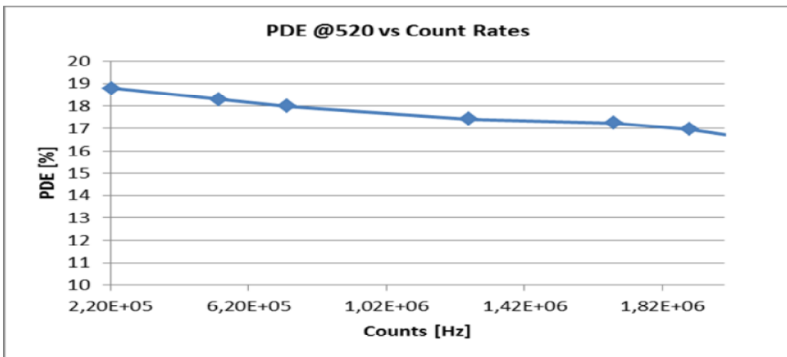
Fig.6 – PDE measurements at 520nm versus counts, from 220 KHz to 1800KHz operating the SiPM at V_{ov}=4V T=25^{\circ}C , V_{thr}=-10 mV, Gate time=90 ns
