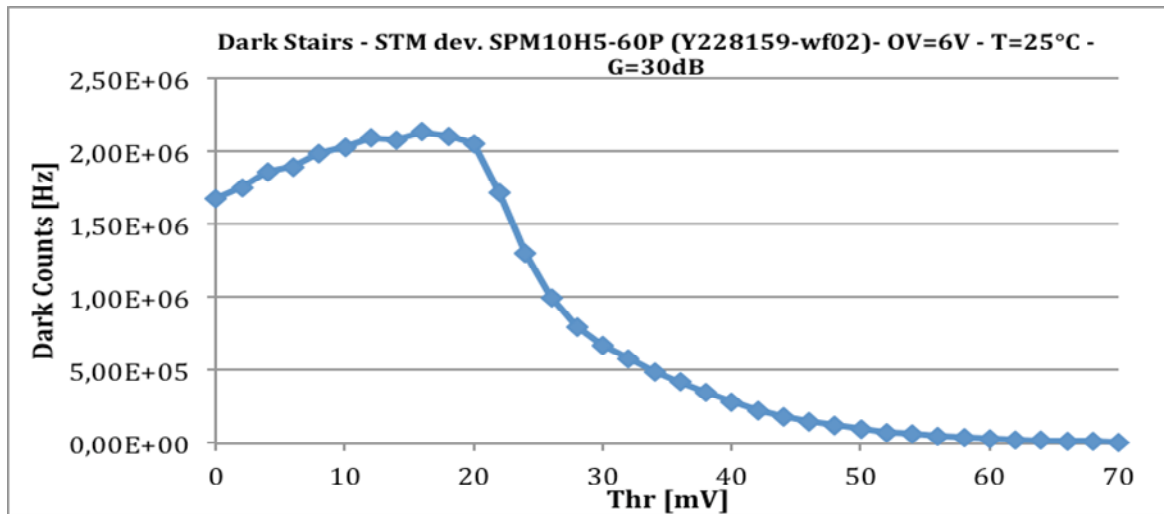
Fig. 14 – Dark Stair versus V_{thr} @ T=25.0^{\circ}C .
