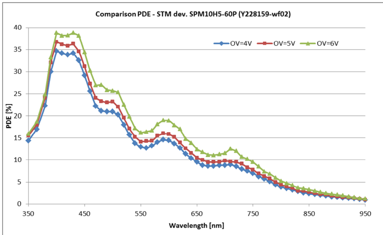
Fig.21– PDE measurements comparison at V_{ov}=4.0V , V_{ov}=5.0V and V_{ov}=6.0V @ T=25^{\circ}C .
