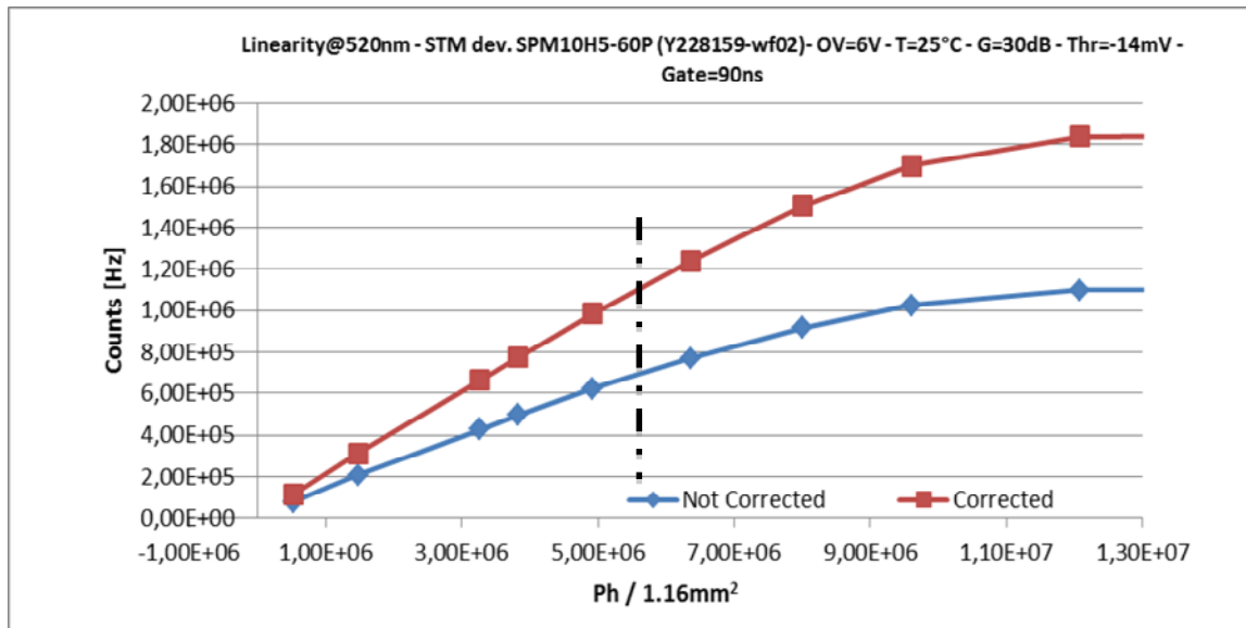
Fig. 17 – Linearity at 520 nm with and without the dead time correction.
