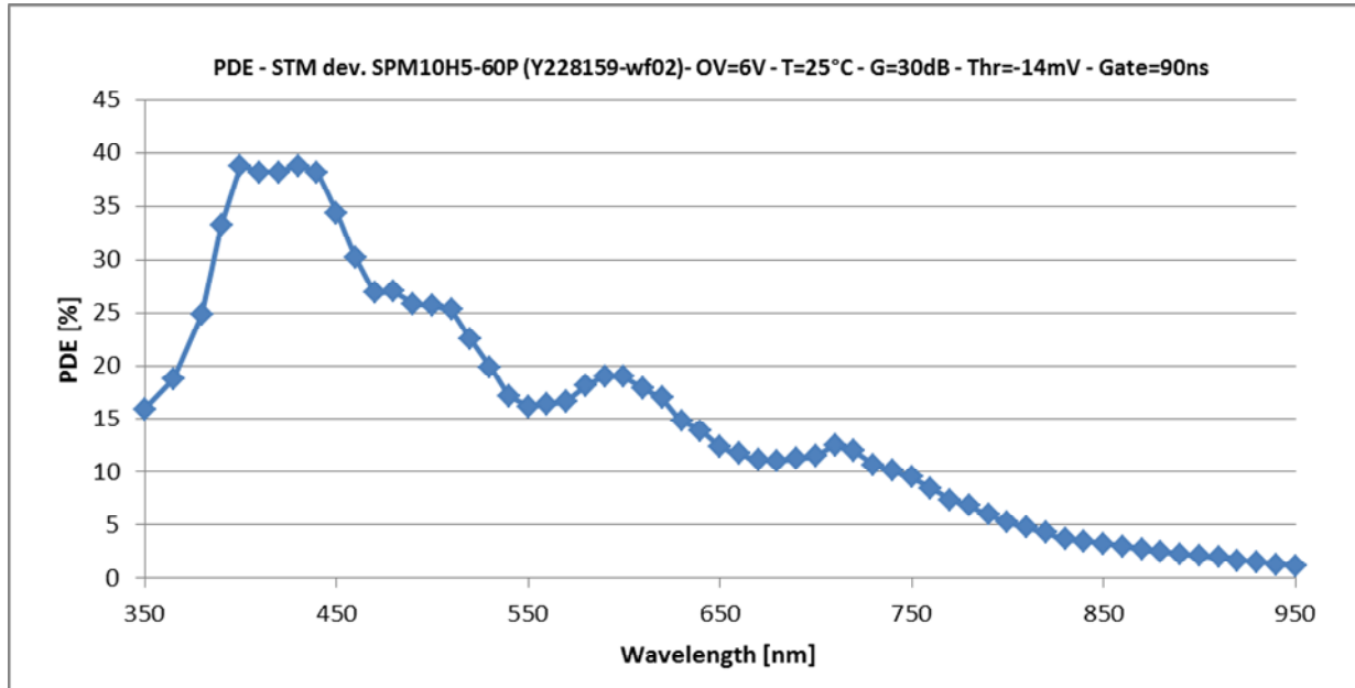
Fig.20 – PDE measurements operating the SiPM at V_{ov}=6V , T=25^{\circ}C , V_{thr}=-14 mV, Gate time=90 ns
