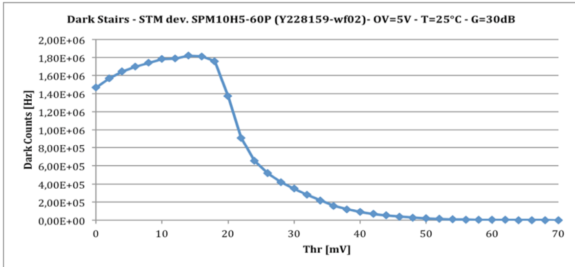
Fig. 8 – Dark Stair versus V_{thr} @ T=25.0^{\circ}C .
