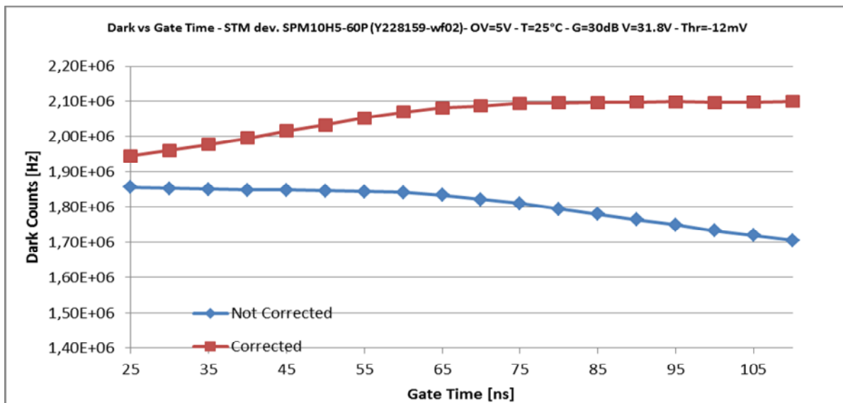
Fig.9 - DARK vs GATE TIME V_{ov}=5V - Thr=-12\text{ mV} T=25^{\circ} . Measurements were performed at gate times from 25ns to 110ns. The upper curve is obtained correcting for dead time the lower curve. Temperature compensation for gain stabilization is also adopted.
