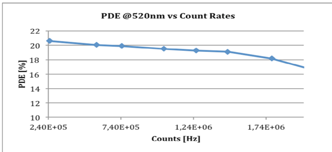
Fig.12 – PDE measurements at 520 nm versus counts from 240KHz to 1700KHz operating the SiPM at V_{ov}=5V T=25^{\circ}C , V_{thr}=-12 mV, Gate time=90 ns
