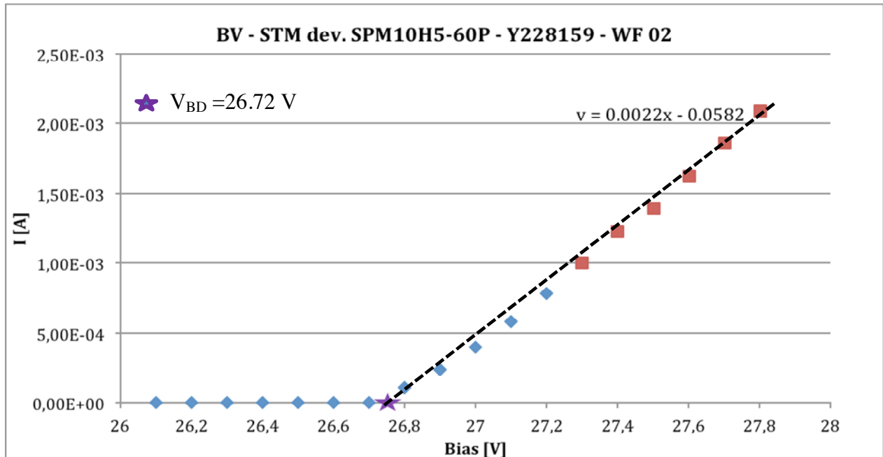
Fig. 1 – BreakDown Voltage @ T=25.0^{\circ}\text{C} .
