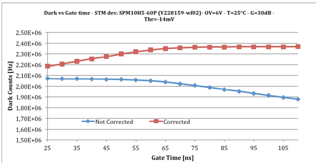
Fig.15 - DARK vs GATE TIME V_{ov}=6V - Thr=-14 mV T=25^{\circ} Measurements were performed at gate times from 25ns to 110ns. The upper curve is obtained correcting for dead time the lower curve. Temperature compensation for gain stabilization is also adopted.
